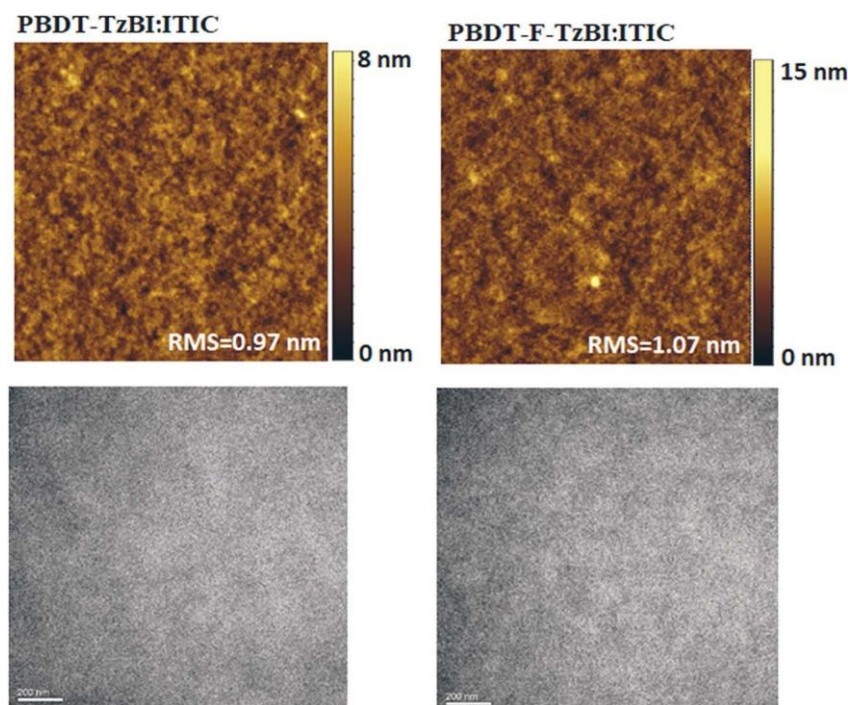
Fig. 3 AFM topography (5 × 5 nm) and TEM images of the optimized PBDT-F-TzBI:ITIC and PBDT-TzBI:ITIC blend films.
