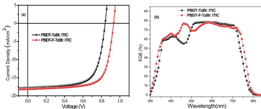
Fig. 2 (a) Current density–voltage characteristics, (b) EQE curves, of PBDT-TzBI:ITIC- and PBDT-F-TzBI:ITIC-based solar cells.
